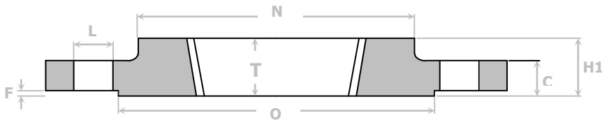
SCREWED FLANGE
