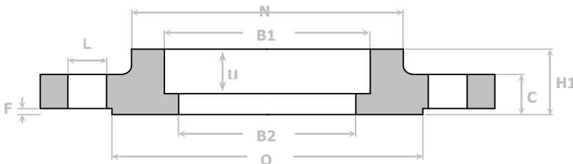
SOCKET WELD FLANGE
