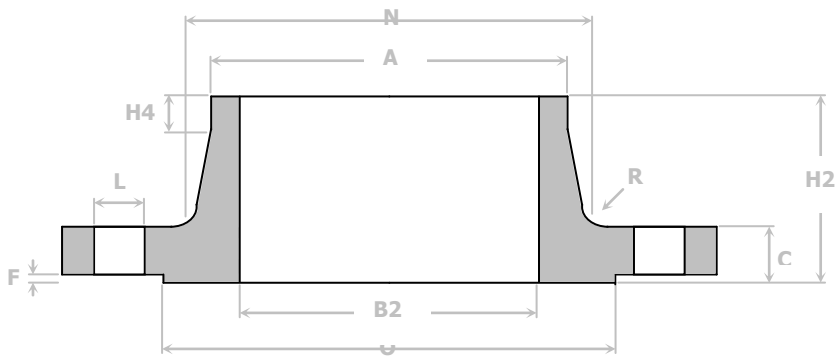
WELD NECK FLANGE
