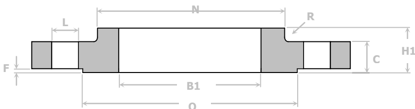
SLIP-ON BOSS FLANGE
